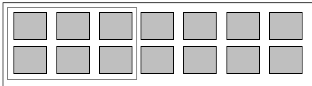
Figure 3. BIO-CEL L-2 arrangement in 20/40 ft HC container (6 / 14 pcs capacity)
