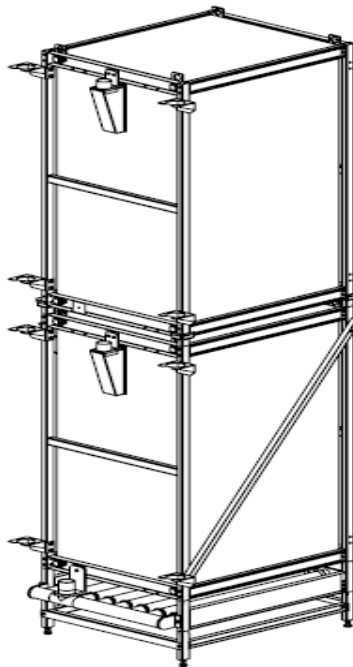
Figure 1. BIO-CEL L-2 Stack scope of supply
