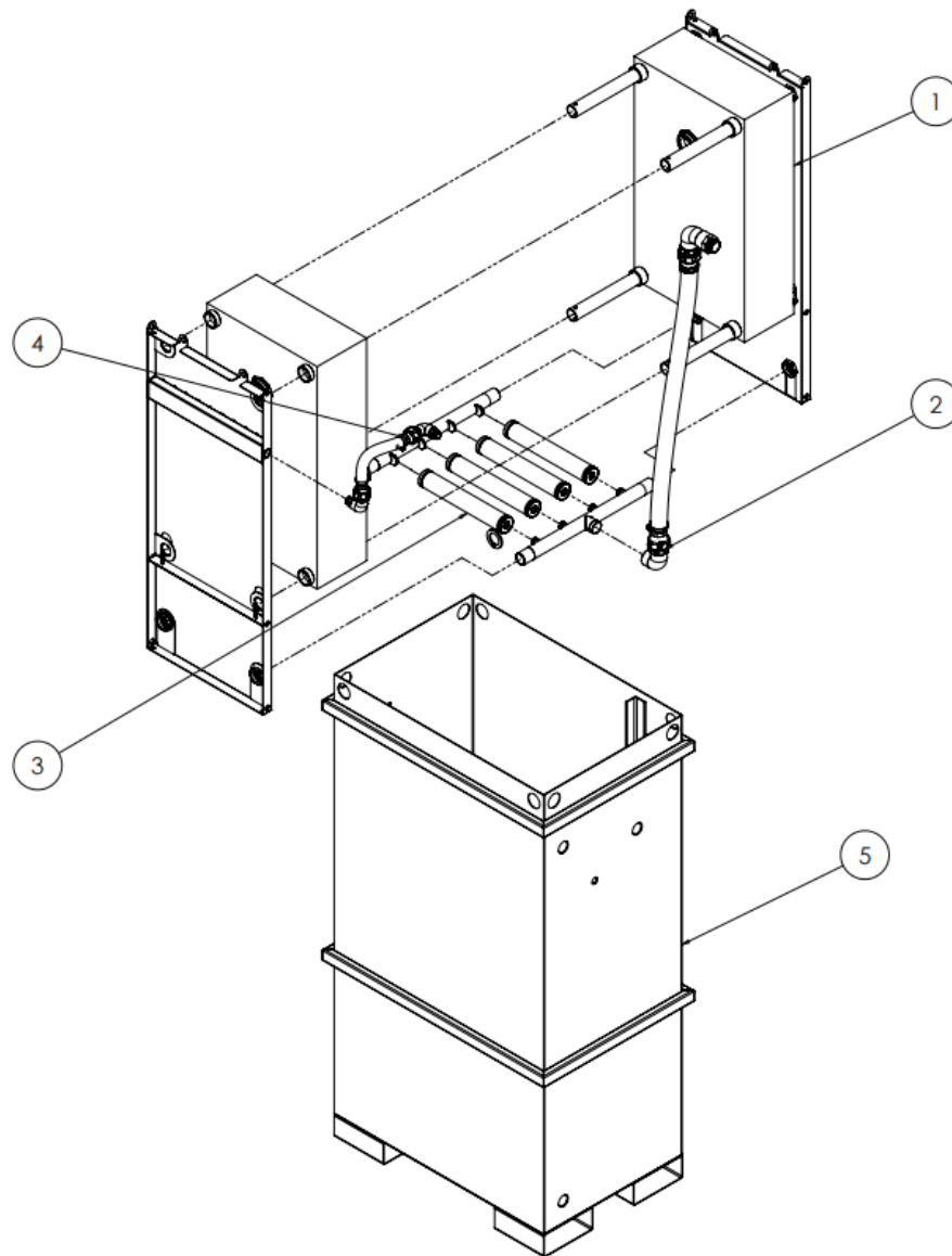
Figure 5. BIO-CEL EASY+ accessories & spare parts
