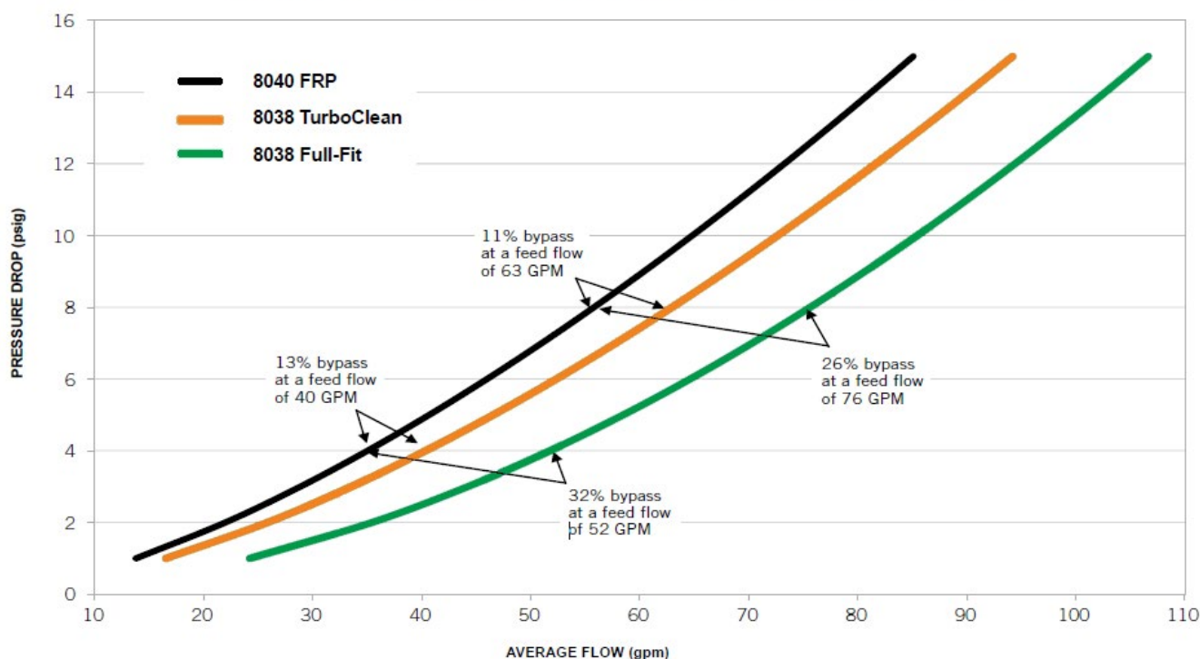
PRESSURE DROP PROFILES OF DIFFERENT 8-INCH ELEMENT EXTERIORS
