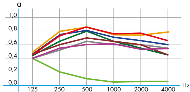
Edge D (rebated and grooved) / S24 Concealed grid For Globe, Quadril and Micro
