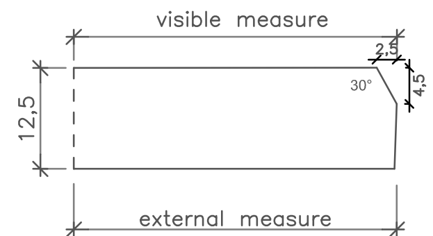
Detail C
