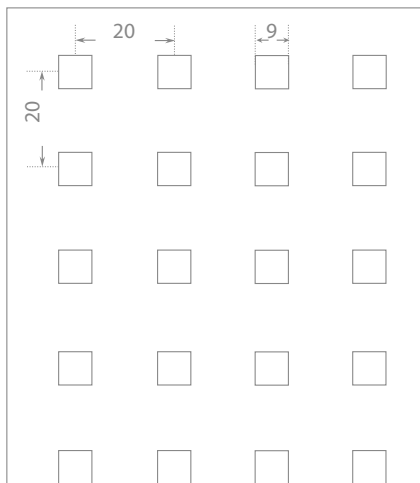
UNITY 9 9x9 mm Perforatiepercentage: 18.9%
