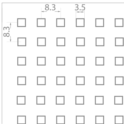
UNITY 3 3.5x3.5 mm Perforatiepercentage: 17.2%
