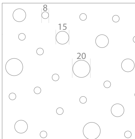
U8 | 15 | 20, Ø8mm, Ø15 mm, Ø20 mm Perforatiepercentage: 10.80%
