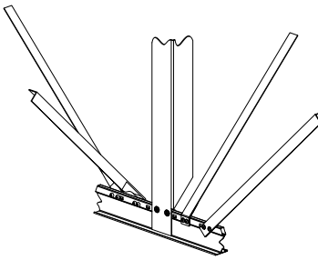
SA55/MT55 diagonal tee option
