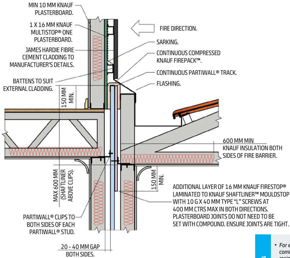
Figure 27: OutRwall Vertical Transition – Any Cladding
