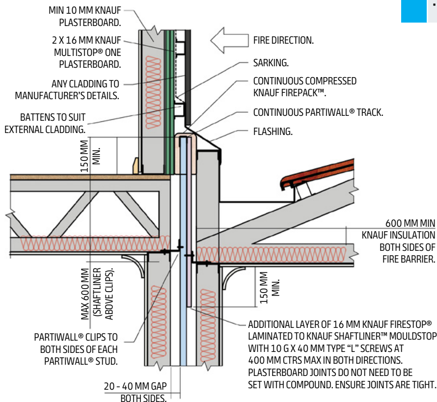
Figure 27: OutRwall Vertical Transition – Any Cladding
