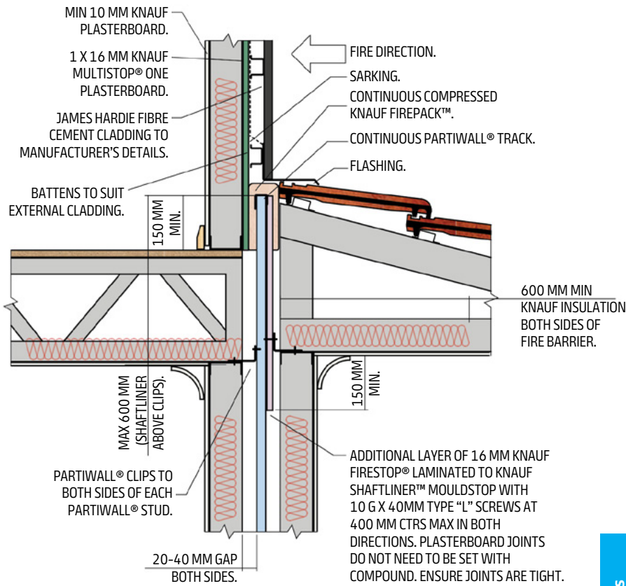
Figure 25: OutRwall Vertical Transition – Any Cladding
