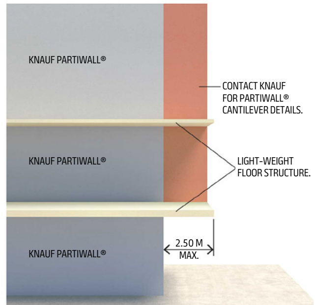
Figure 1: Cantilever PartiWall
