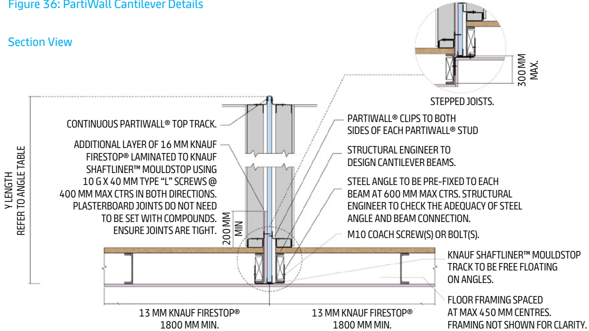
Figure 36: PartiWall Cantilever Details
