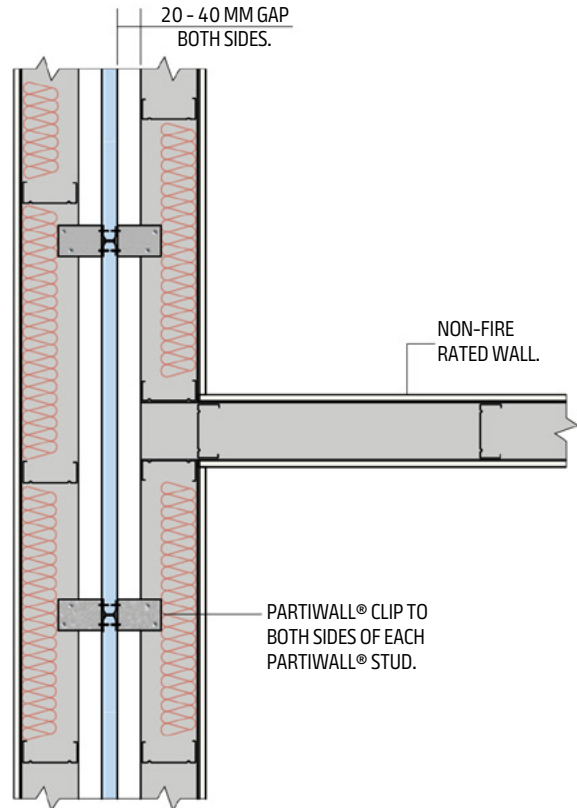
Figure 29: Internal Wall Junction – Plan View
