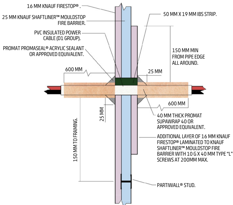
Figure 43: Power Cable Penetration at Roof Space – FRL -/60/60
