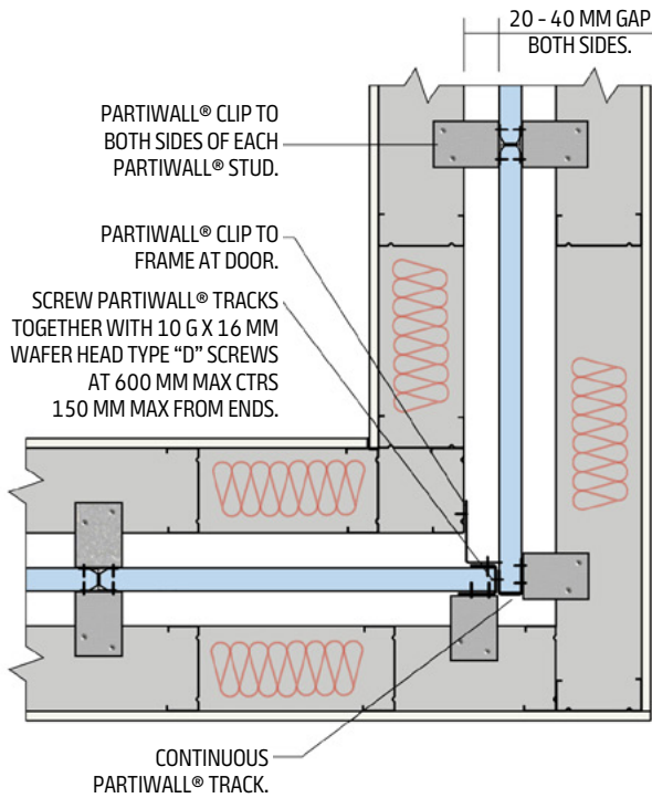
Figure 28: Typical Corner – Plan View
