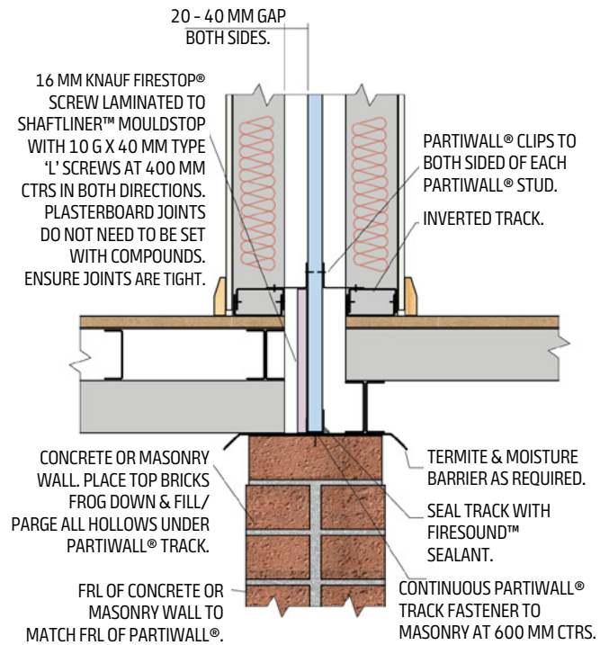
Figure 10: Masonry Base
