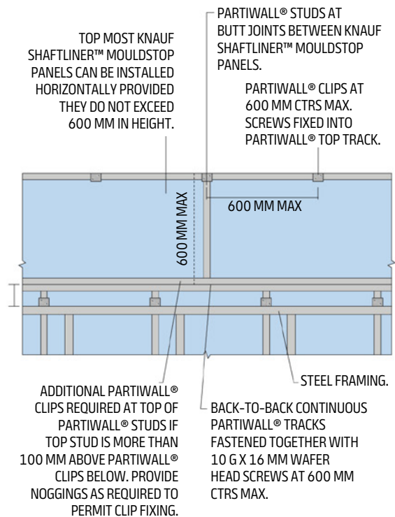
Figure 21: Horizontal Shaftliner MouldStop Under Roof
