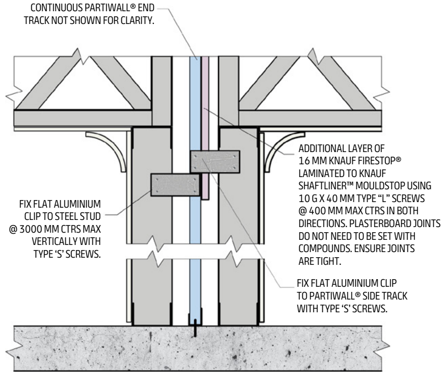
Figure 39: Flat Aluminium Clip Detail
