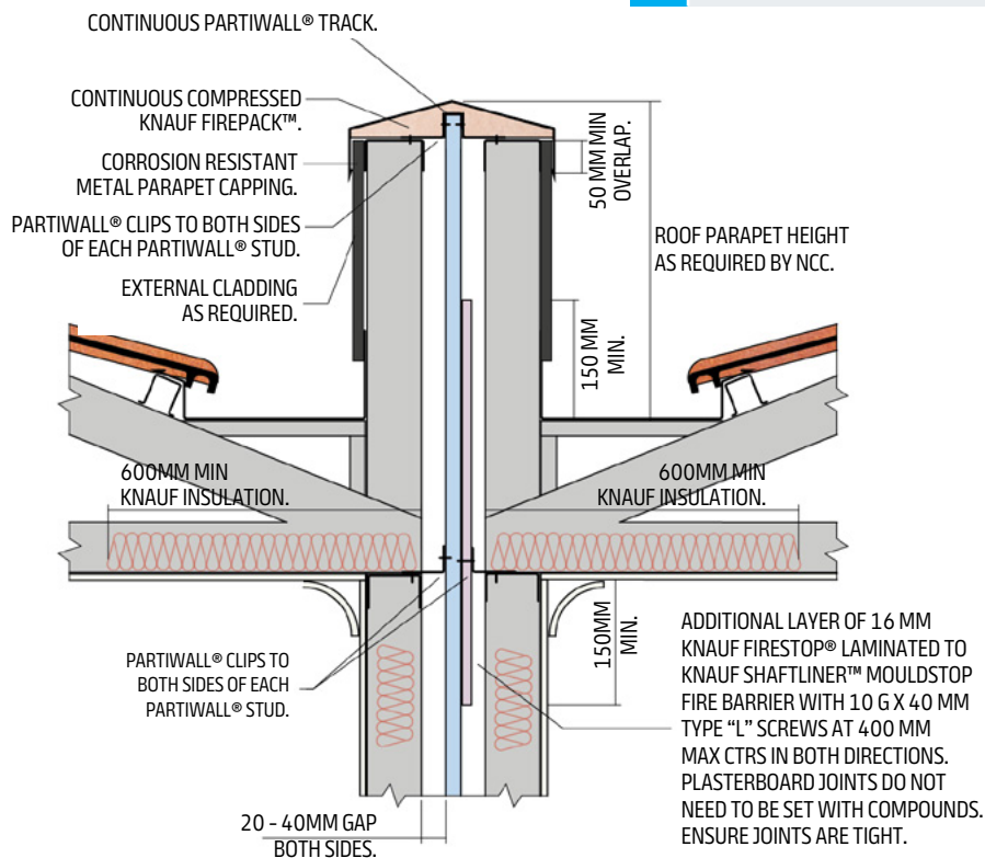
Figure 17: Parapet Roof Junction
