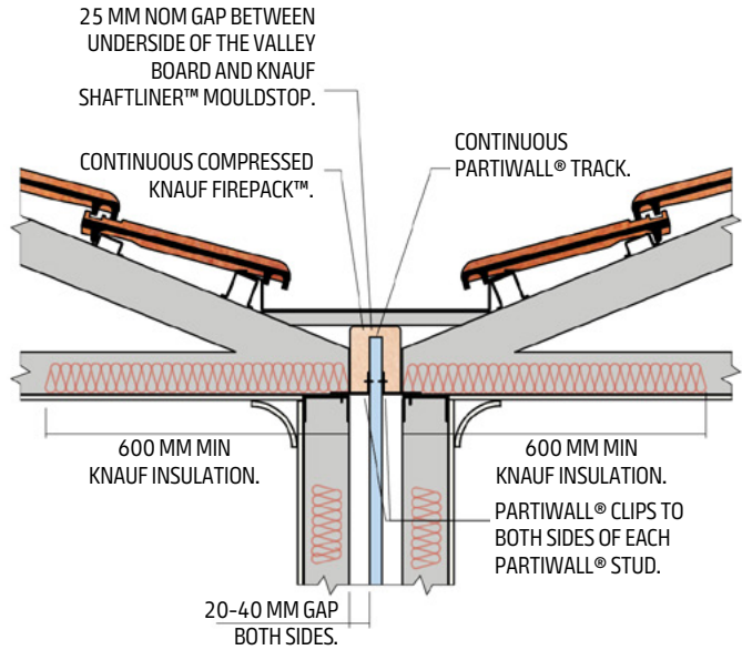
Figure 19: Roof Box Gutter
