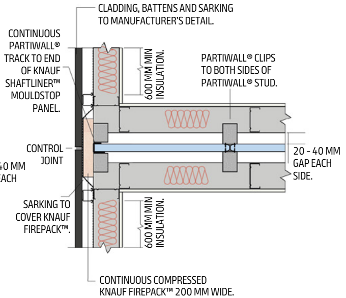
Figure 36: Clad Wall Junction with Thermal Break – Plan View
