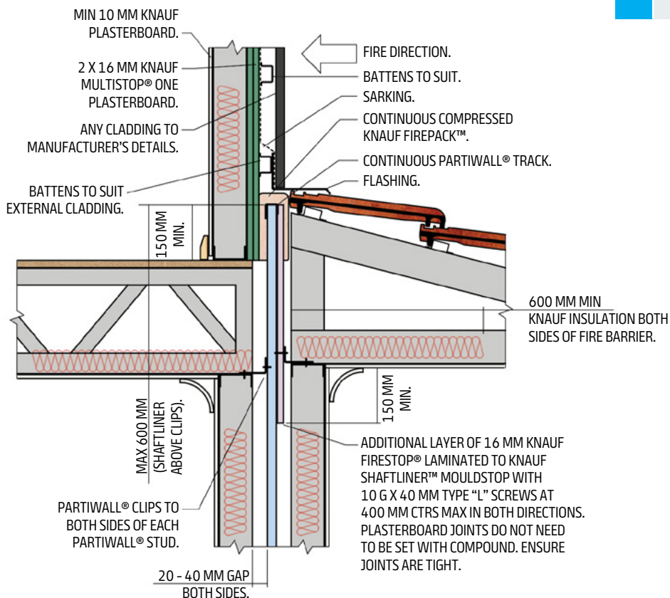
Figure 25: OutRwall Vertical Transition – Any Cladding
