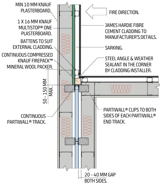
Figure 33: OutRwall Horizontal Transition – JH Cladding
