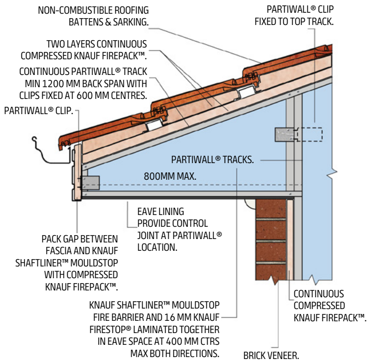
Figure 23: Eave Closure – Section View
