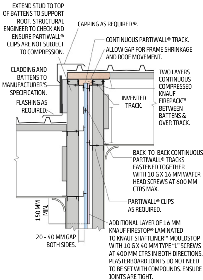
Figure 20: Staggered Metal Roof
