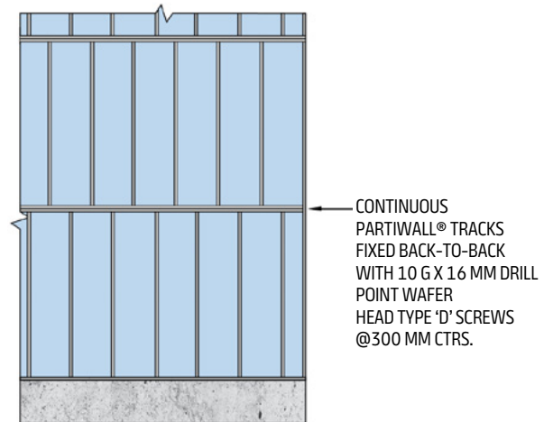
Figure 8: PartiWall H-Studs Staggered
