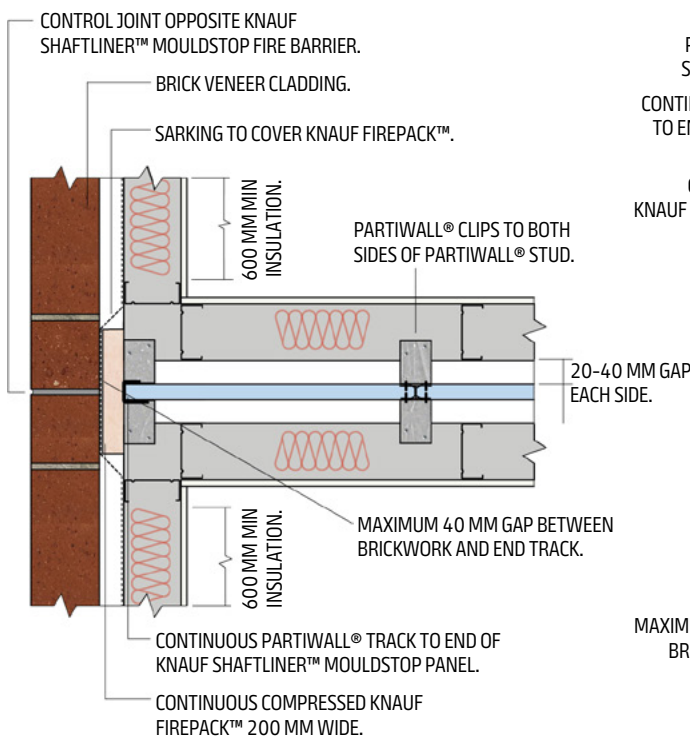
Figure 37: Brick Veneer Wall Junction 1 – Plan View
