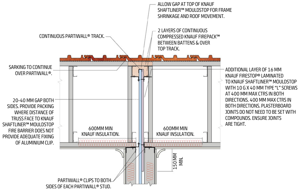
Figure 16: Pitched Roof Junction
