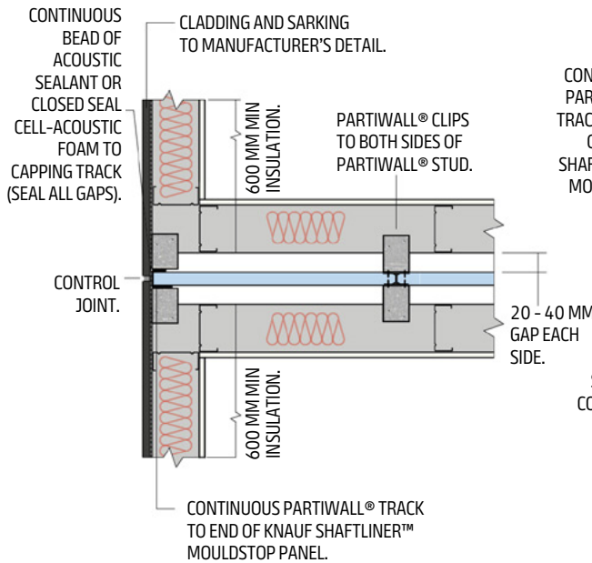
Figure 35: Clad Wall Junction – Plan View
