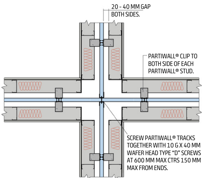
Figure 30: 4 Way Intersecting Wall – Plan View
