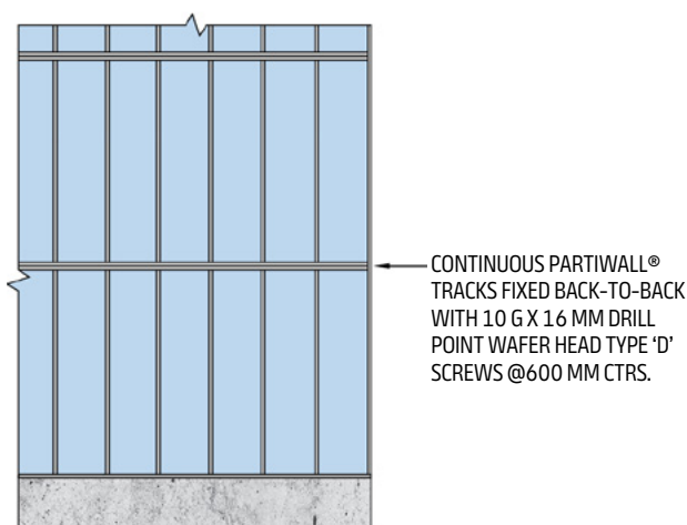
Figure 7: PartiWall H-Studs Aligned
