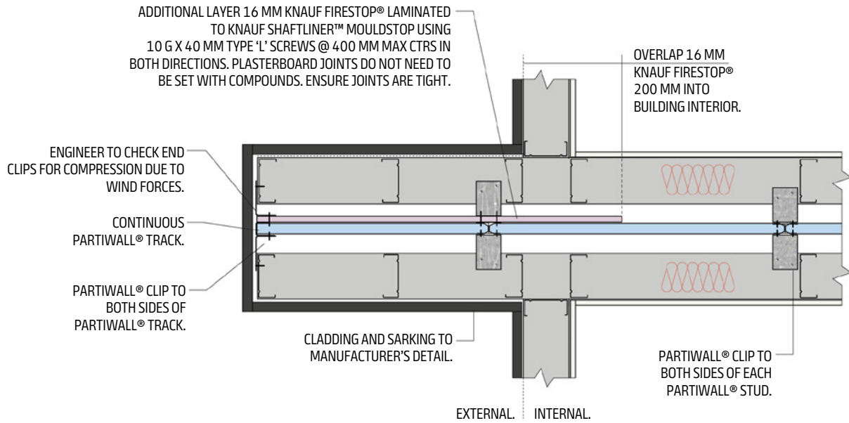
Figure 32: External to Internal PartiWall – Plan View
