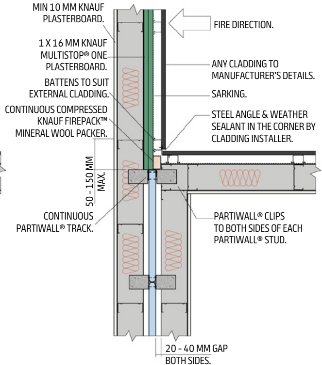
Figure 34: OutRwall Horizontal Transition – Any Cladding
