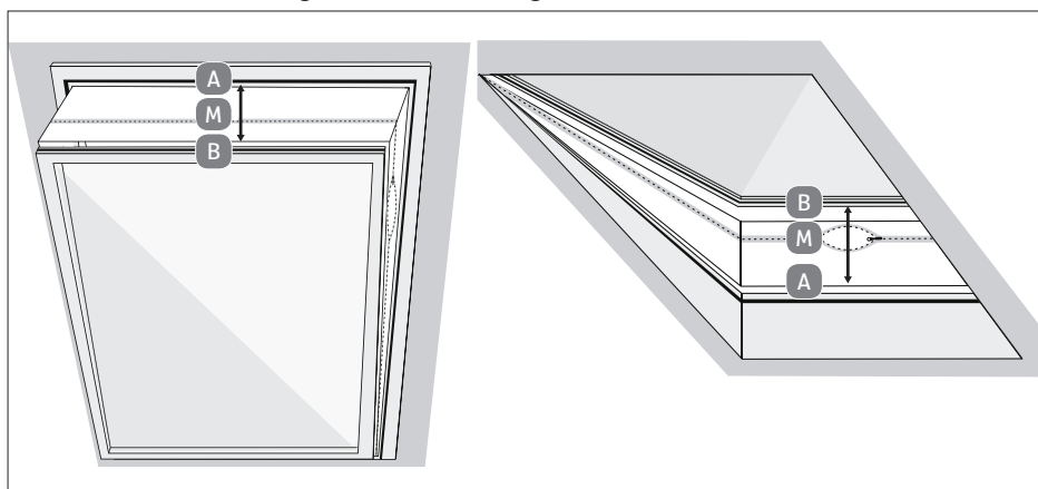
Fig. 13 – Roof window installation
