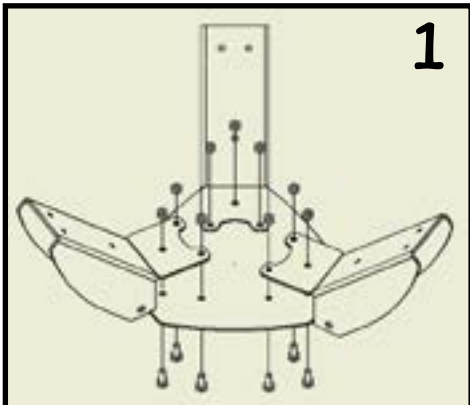
FIRE PIT - style 890
