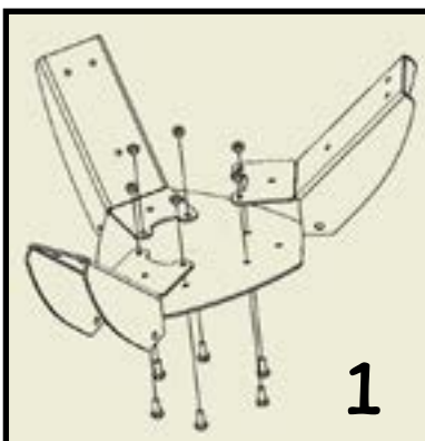
FIRE PIT - style 890, with a support frame
